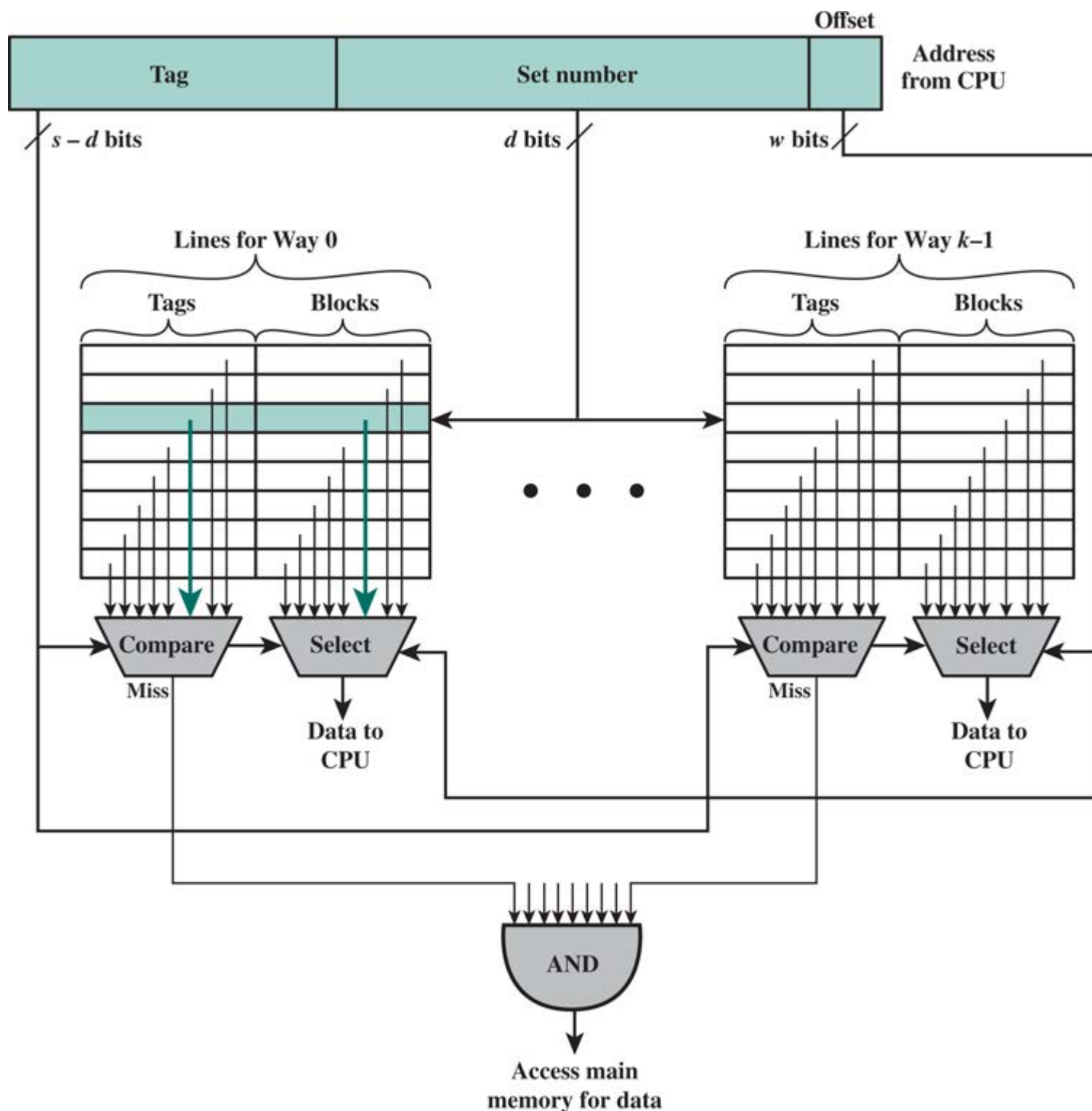
Figure 5.13 k -Way Set Associative Cache Organization
