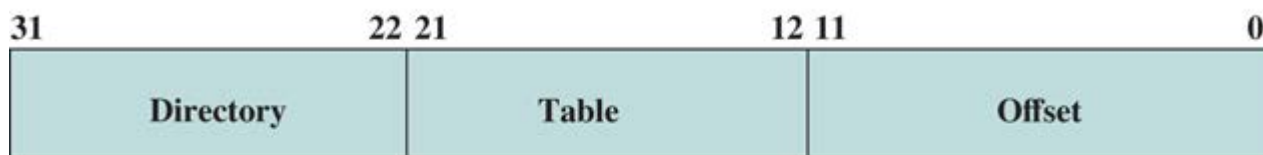
(b) Linear address
