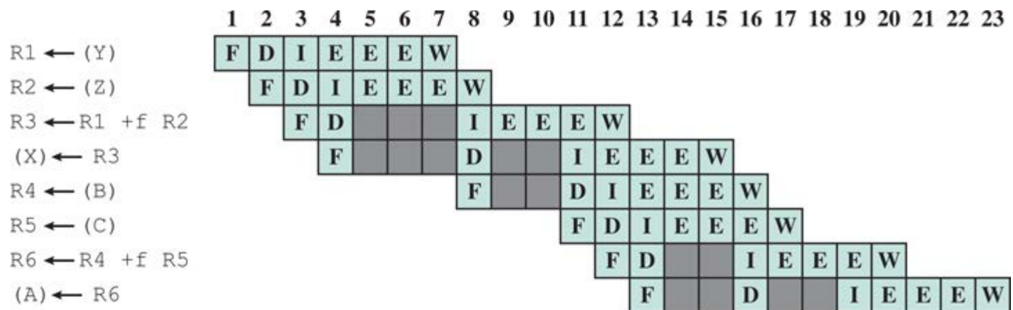
(a) In-order instruction issuing
