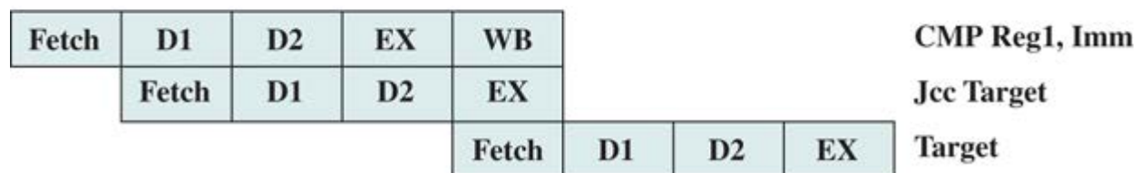
(c) Branch instruction timing
