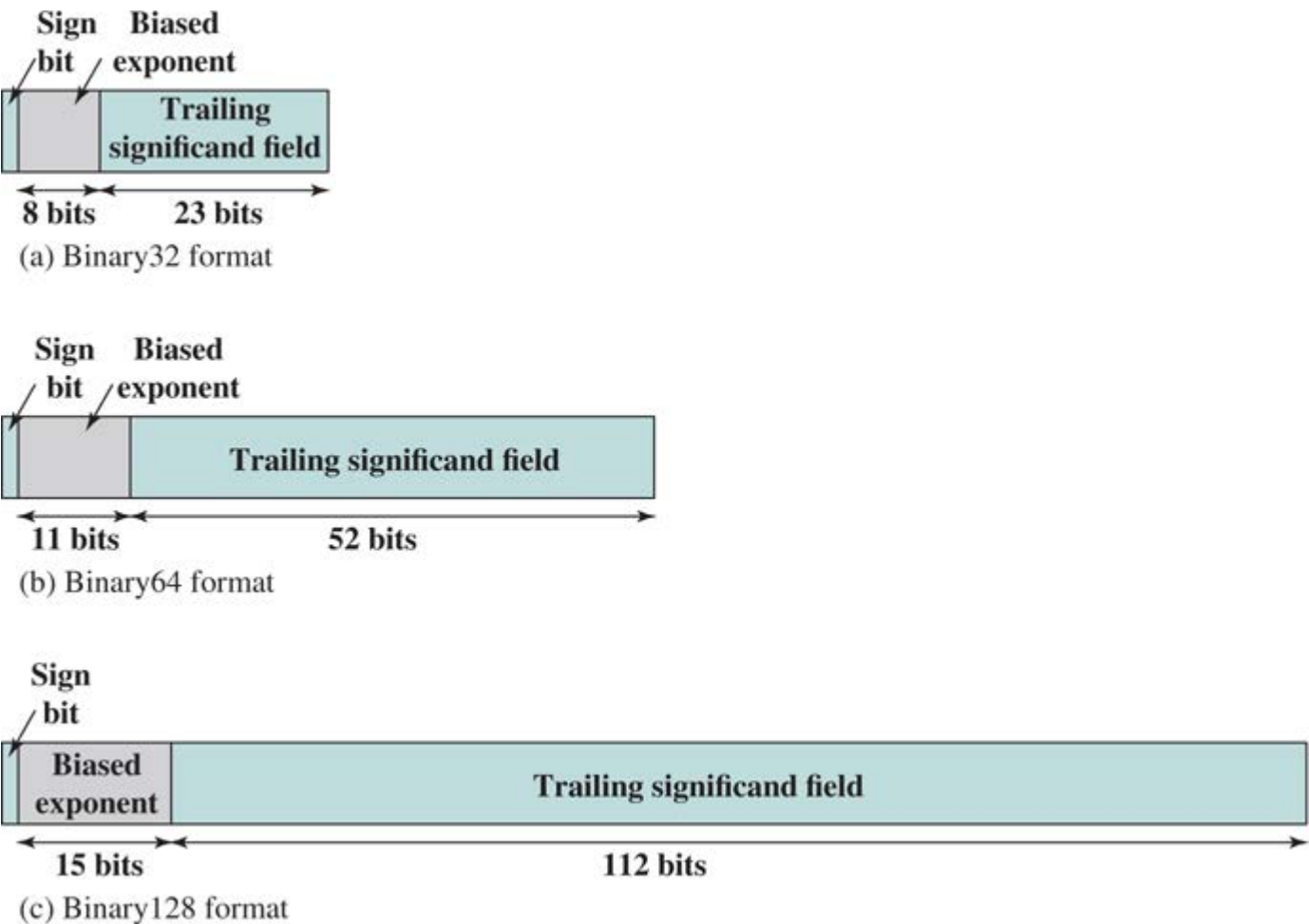
Figure 11.21 IEEE 754 Formats
