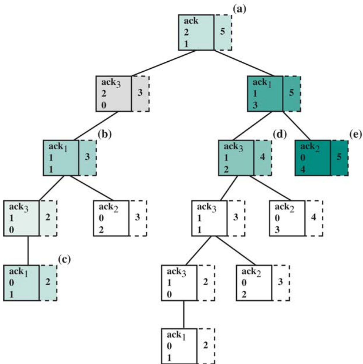
(b) Activation tree for Ackermann (2, 1)
