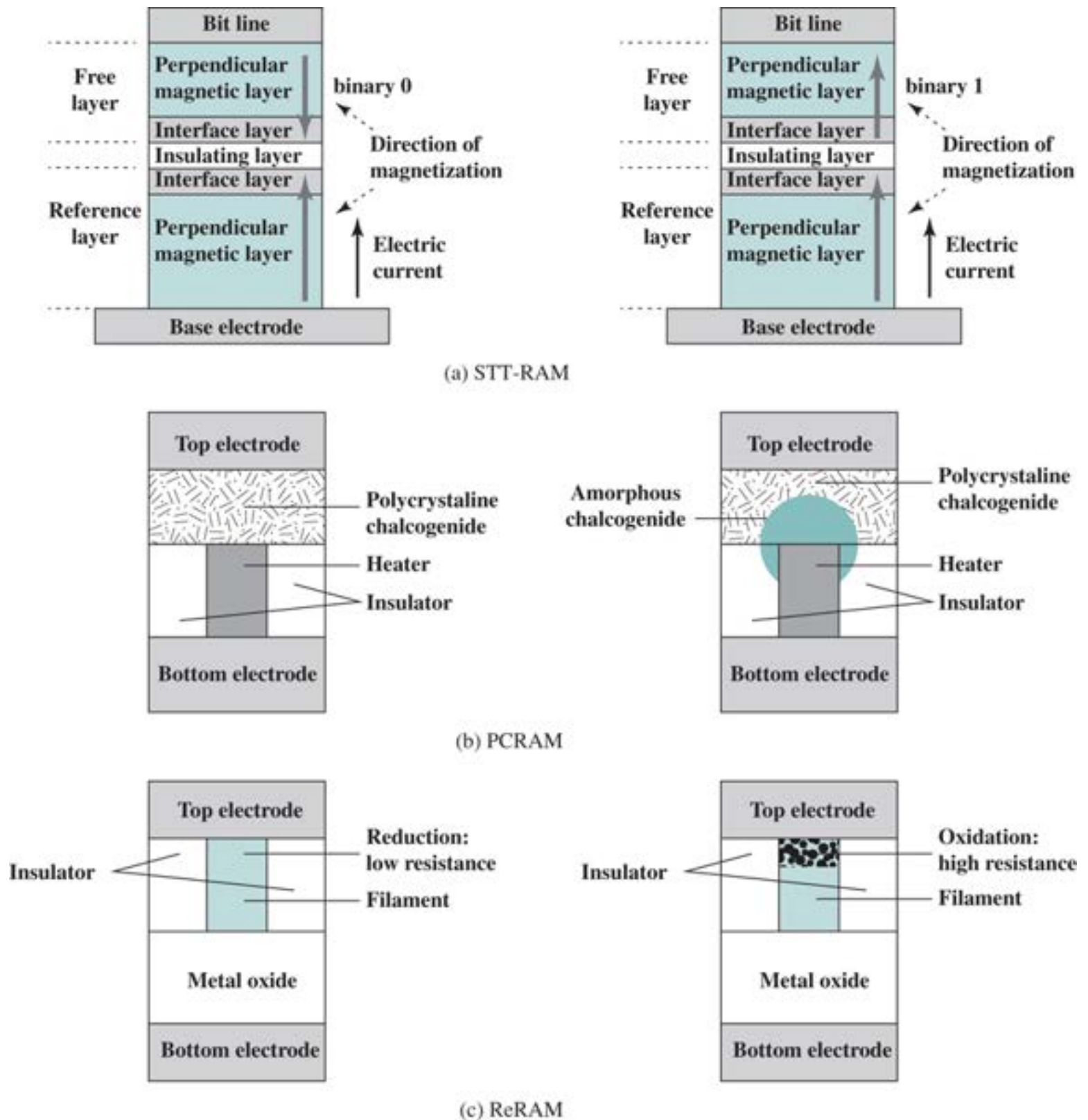
Figure 6.21 Nonvolatile RAM Technologies
