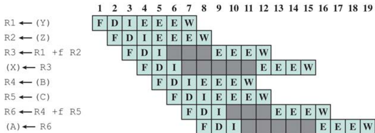
(c) Hardware scoreboard for dynamic instruction scheduling
