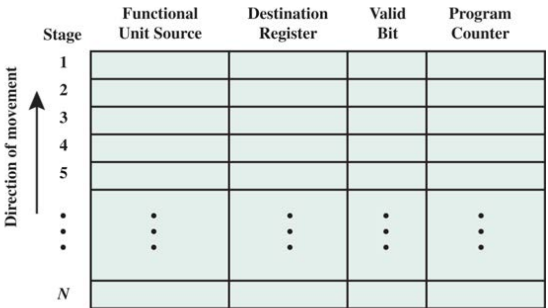
Figure G.8 Result Shift Register
