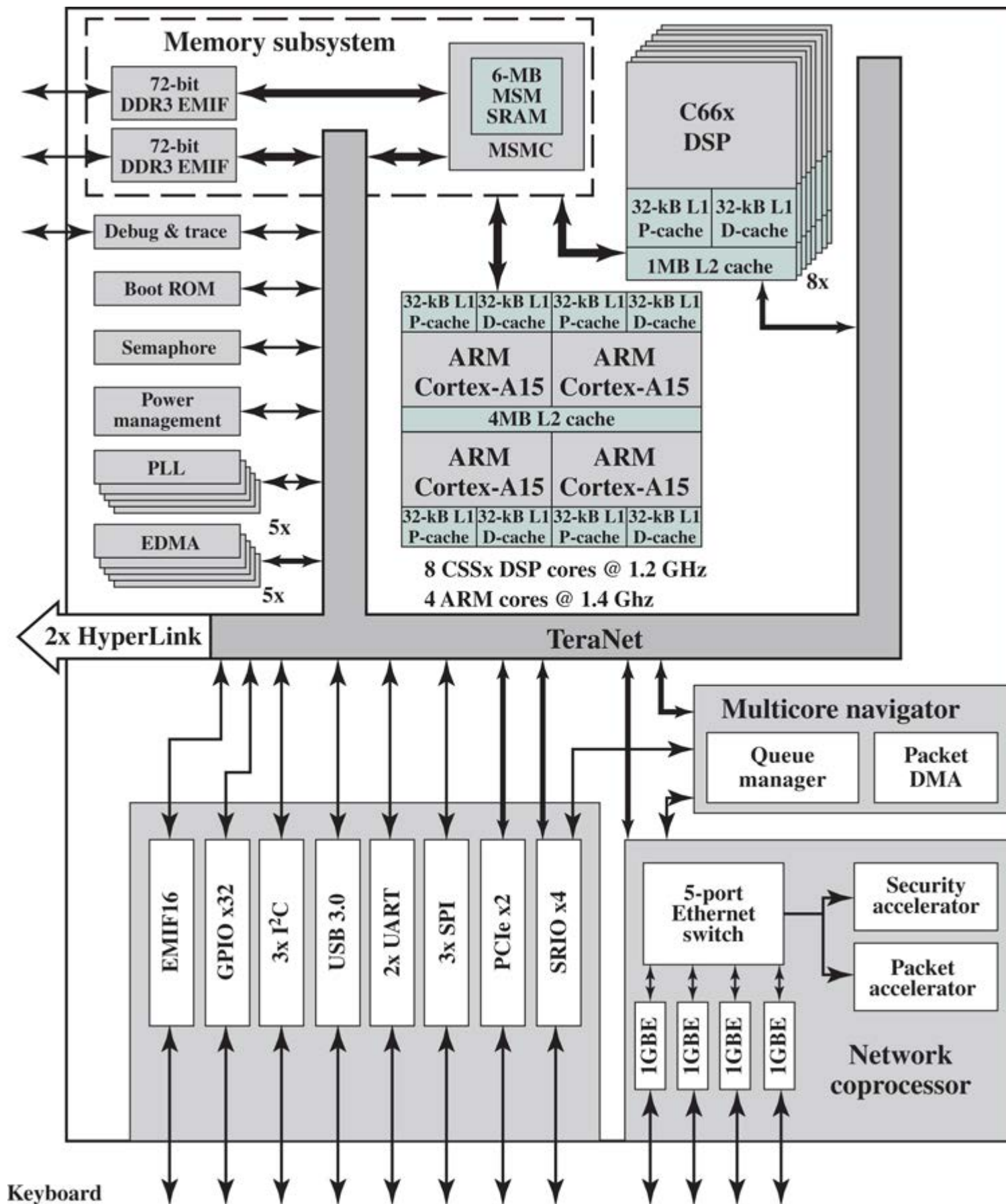
Figure 21.8 Texas Instruments 66AK2H12 Heterogenous Multicore Chip
