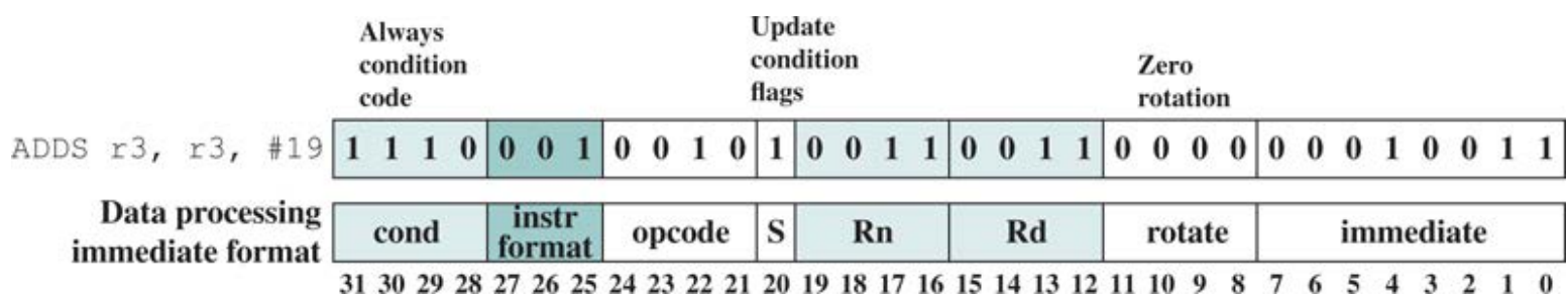
Figure 15.9 Translating an ARM Assembly Instruction into a Binary Machine Instruction
