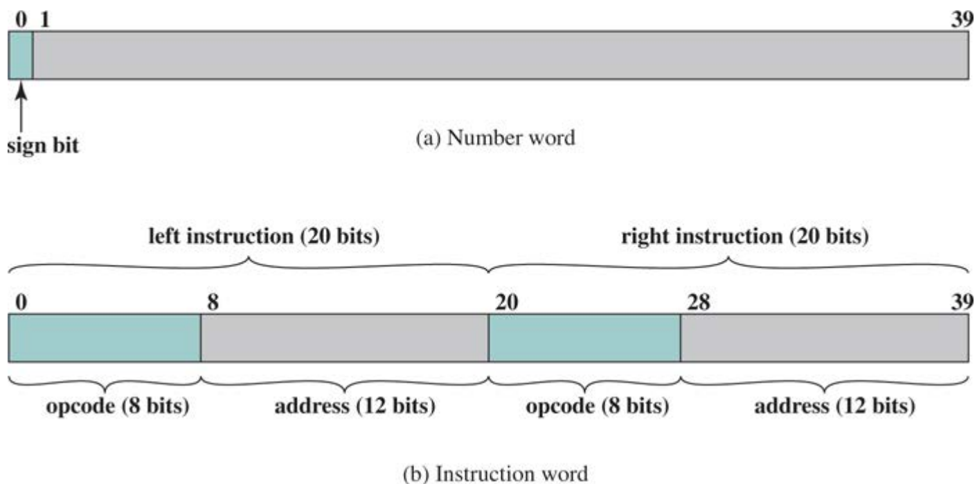
Figure 1.7 IAS Memory Formats
