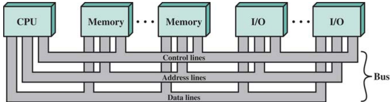
Figure A.1 Bus Interconnection Scheme
