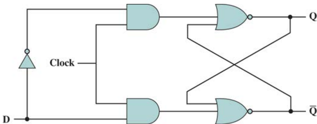
Figure 12.27 D Flip-Flop
