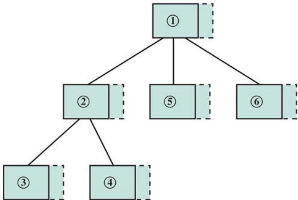
(a) Activation record instance
