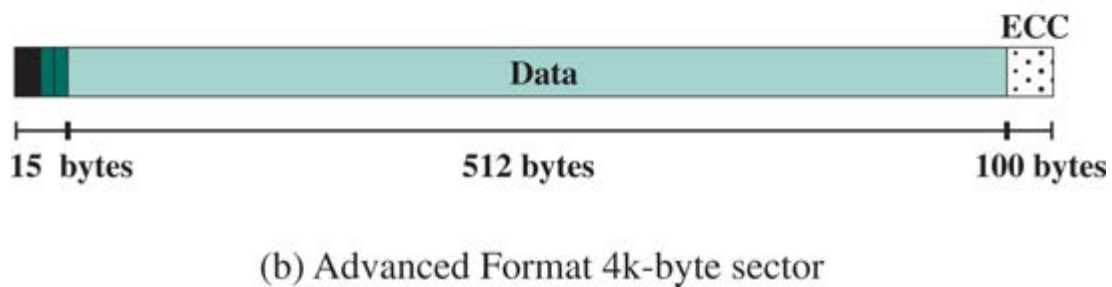
Figure 7.4 Legacy and Advanced Sector Formats
