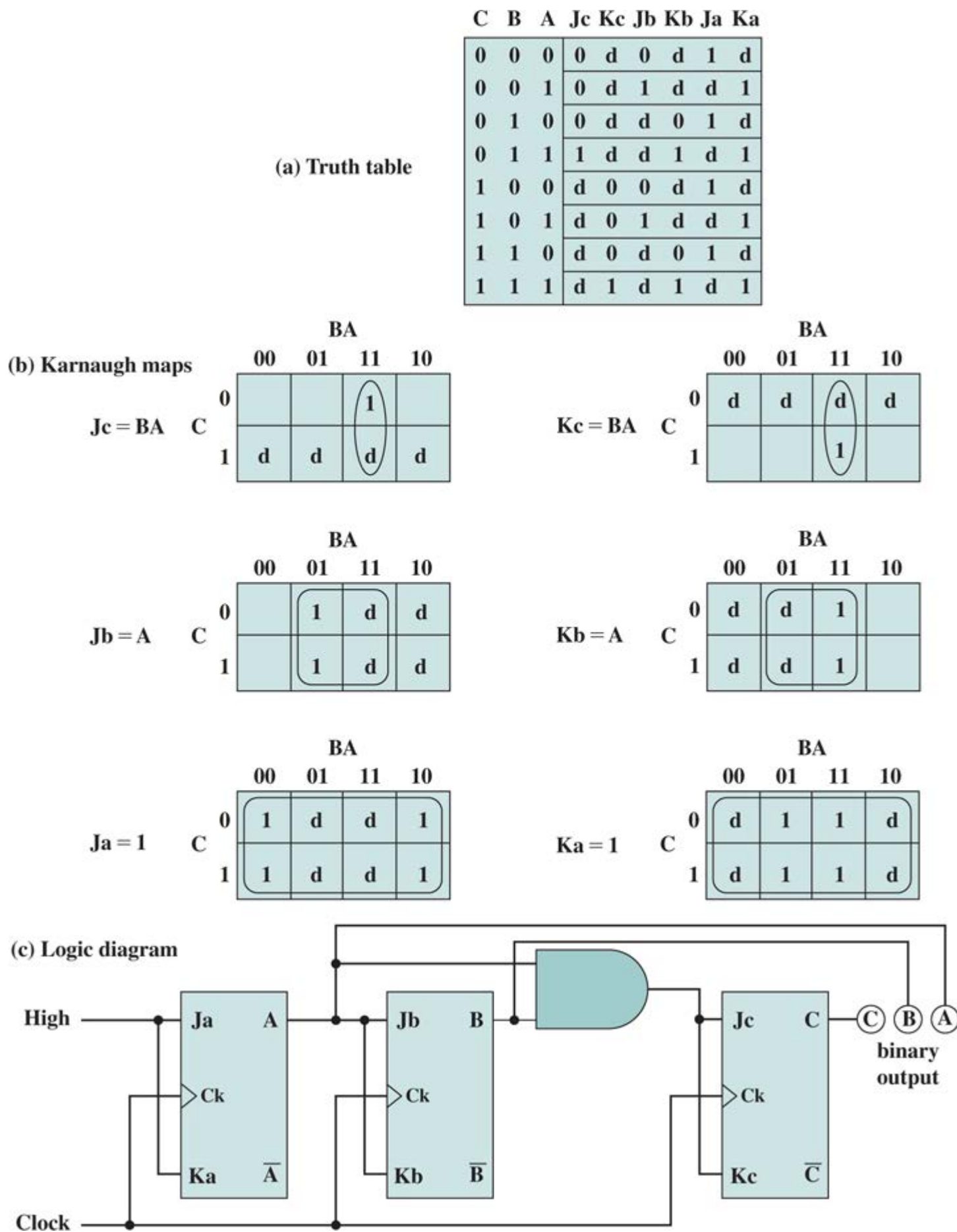
Figure 12.33 Design of a Synchronous Counter
