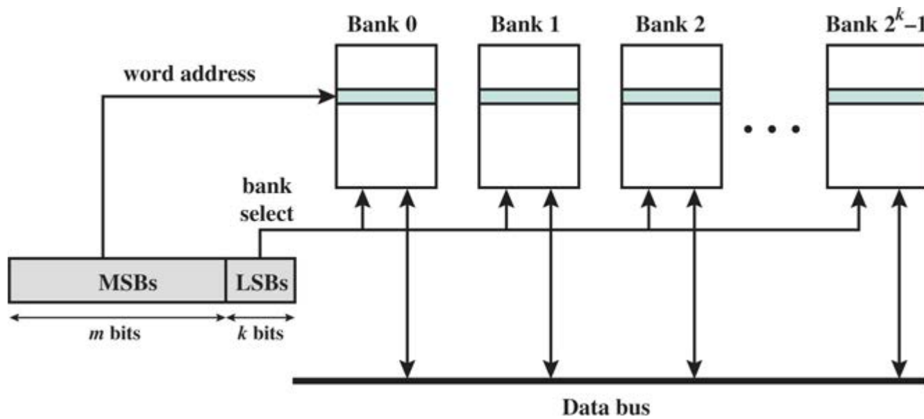
Figure C.2 Interleaved Memory
