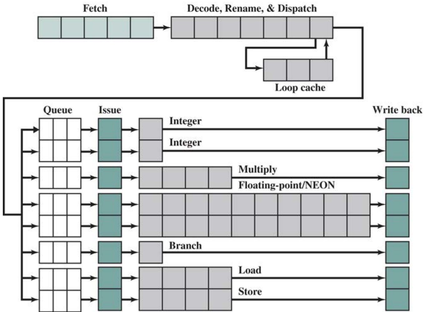
(b) Cortex A-15 Pipeline
