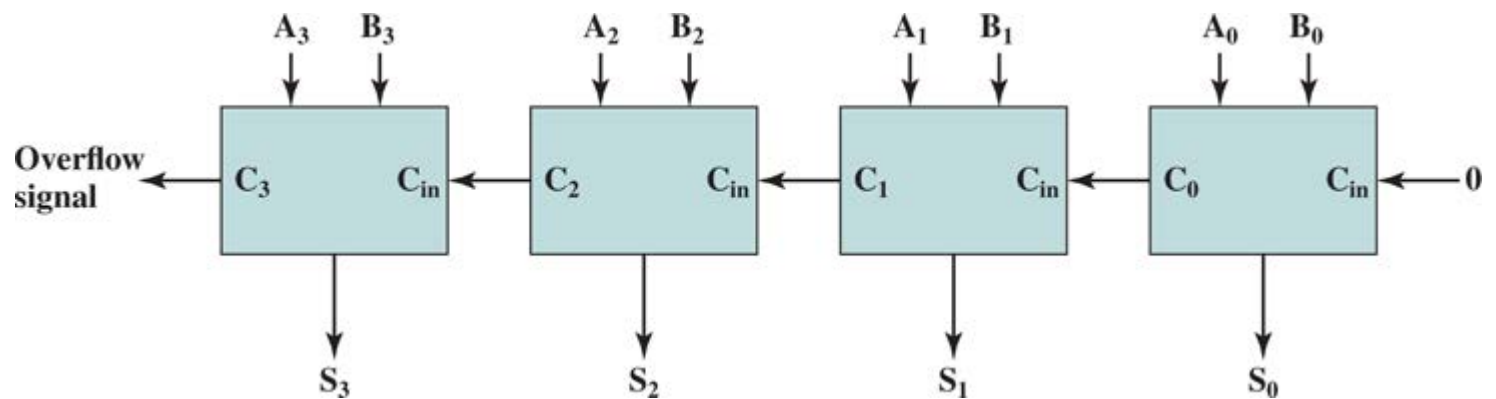
Figure 12.21 4-Bit Adder
