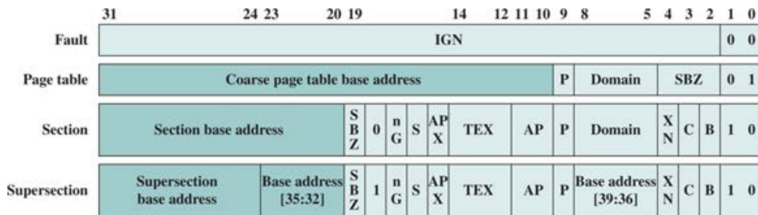
(a) Alternative first-level descriptor formats
