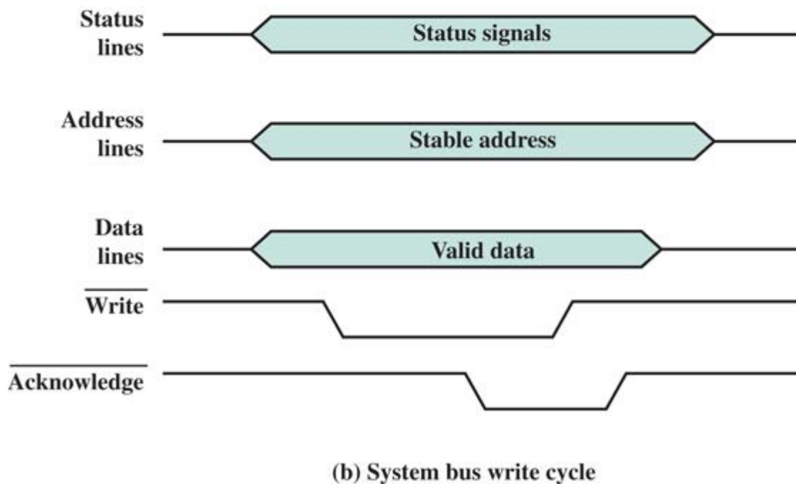
Figure A.4 Timing of Asynchronous Bus Operations
