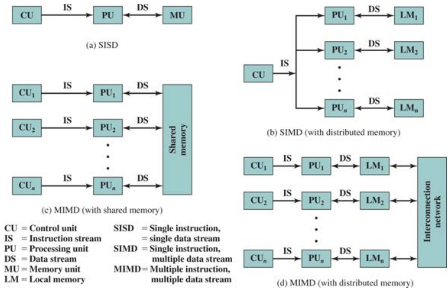
Figure 20.2 Alternative Computer Organizations
