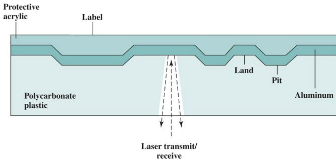
Figure 7.9 CD Operation
