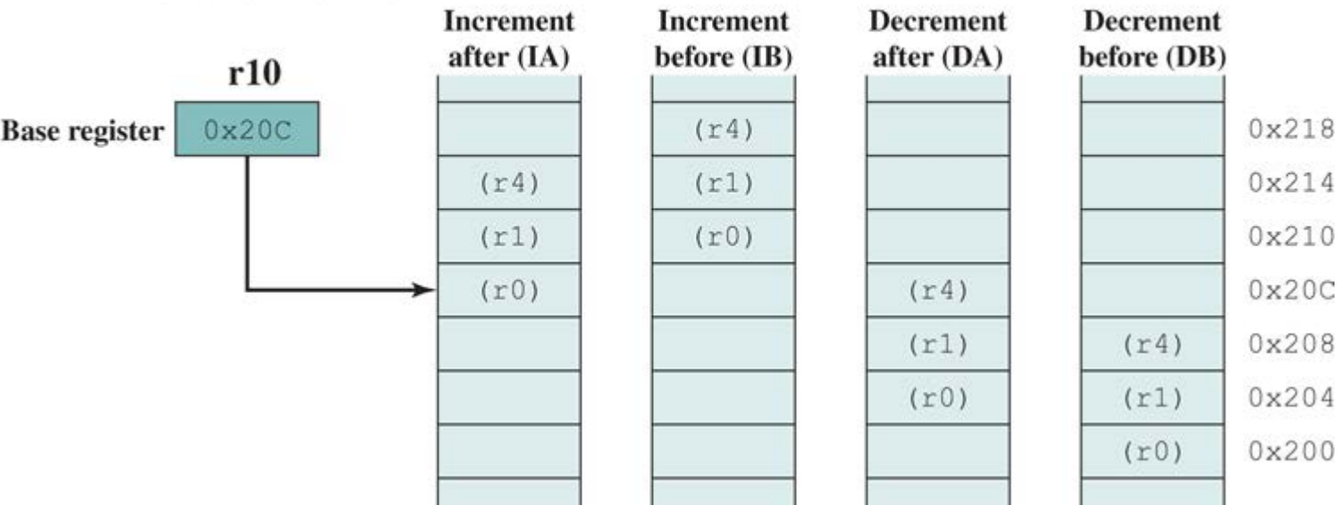
Figure 14.4 ARM Load/Store Multiple Addressing
