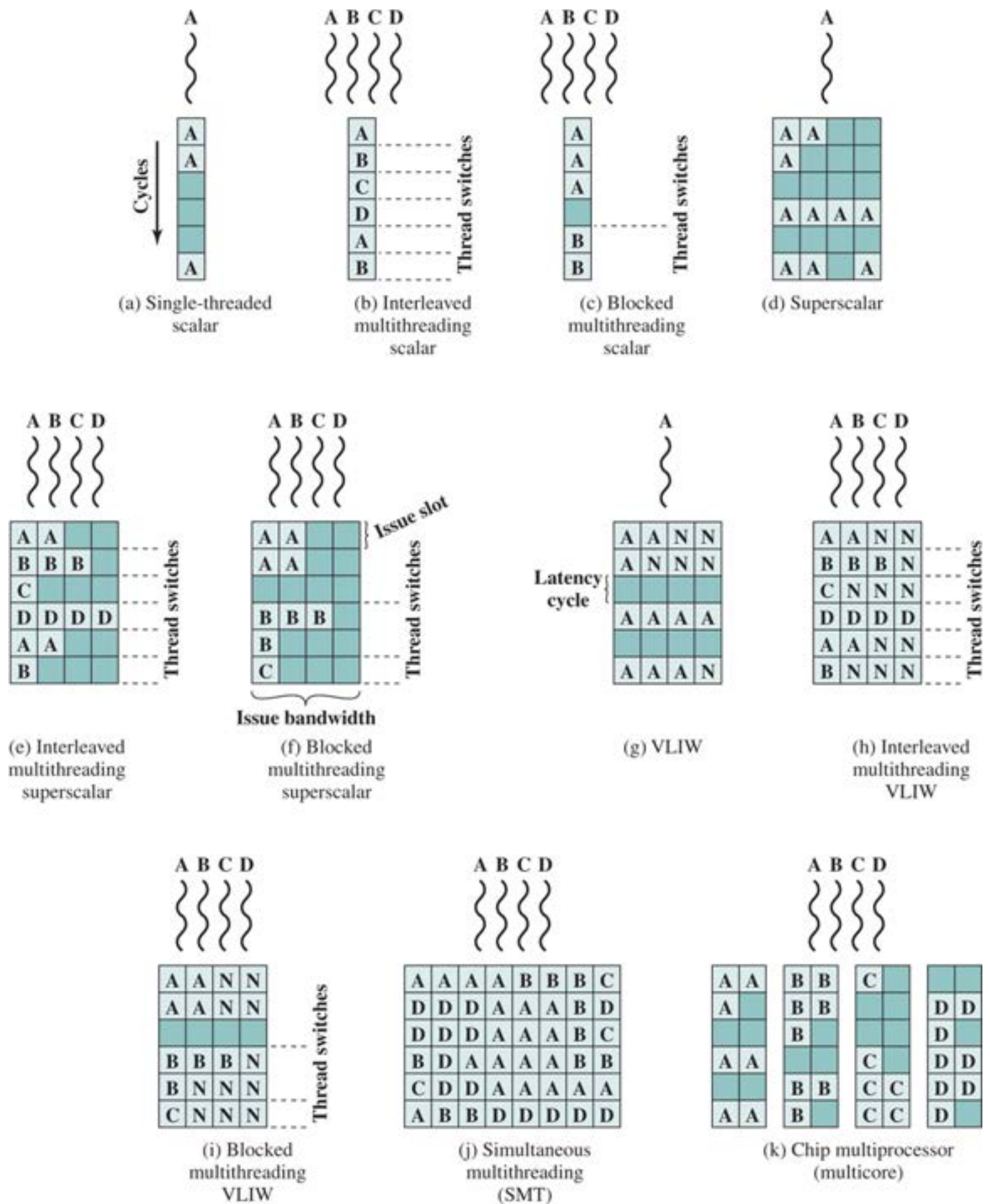
Figure 20.10 Approaches to Executing Multiple Threads
