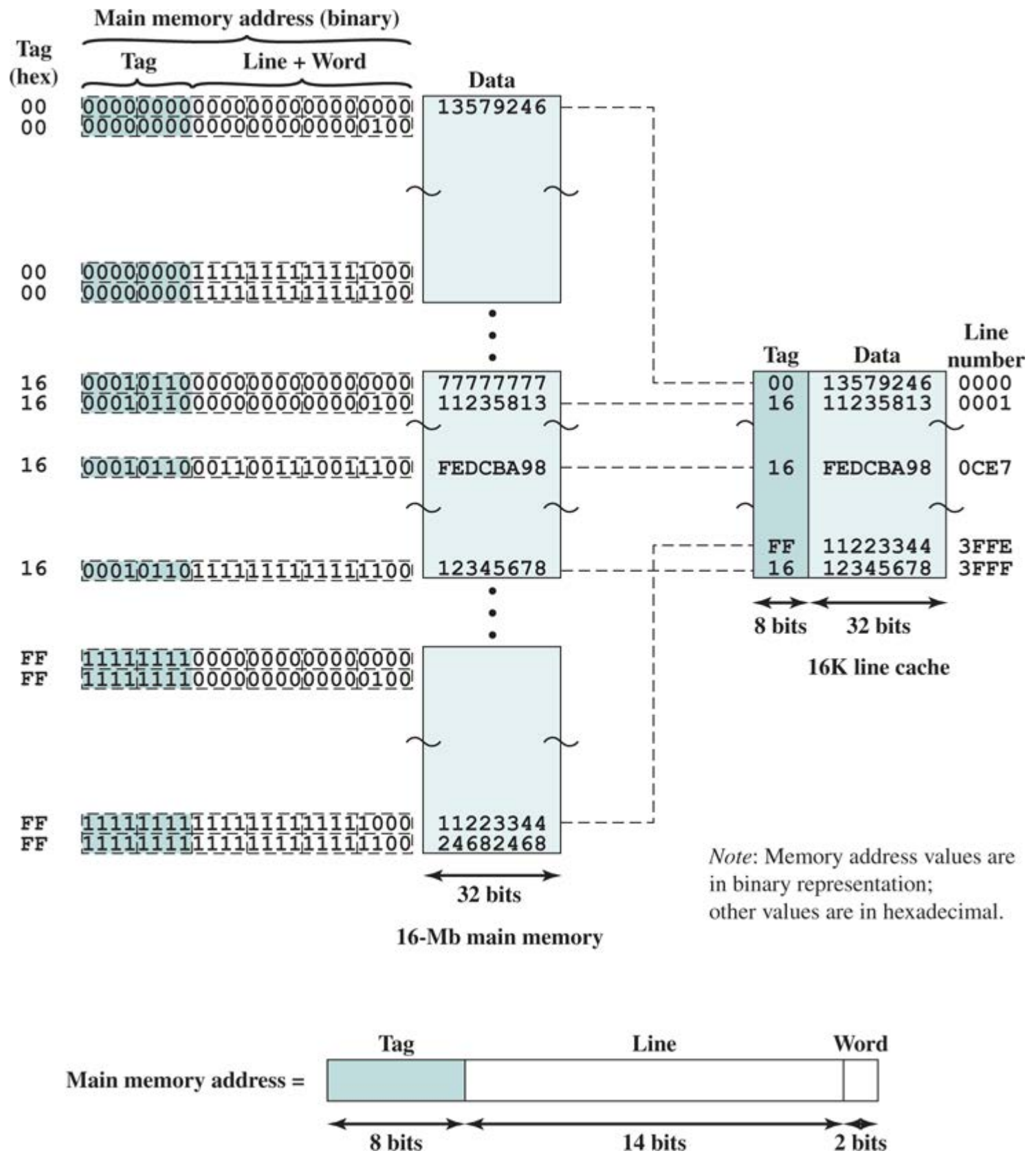
Figure 5.8 Direct Mapping Example
