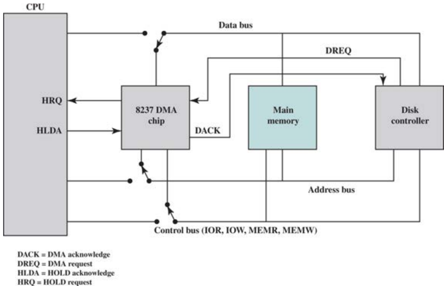
Figure 8.15 8237 DMA Usage of System Bus
