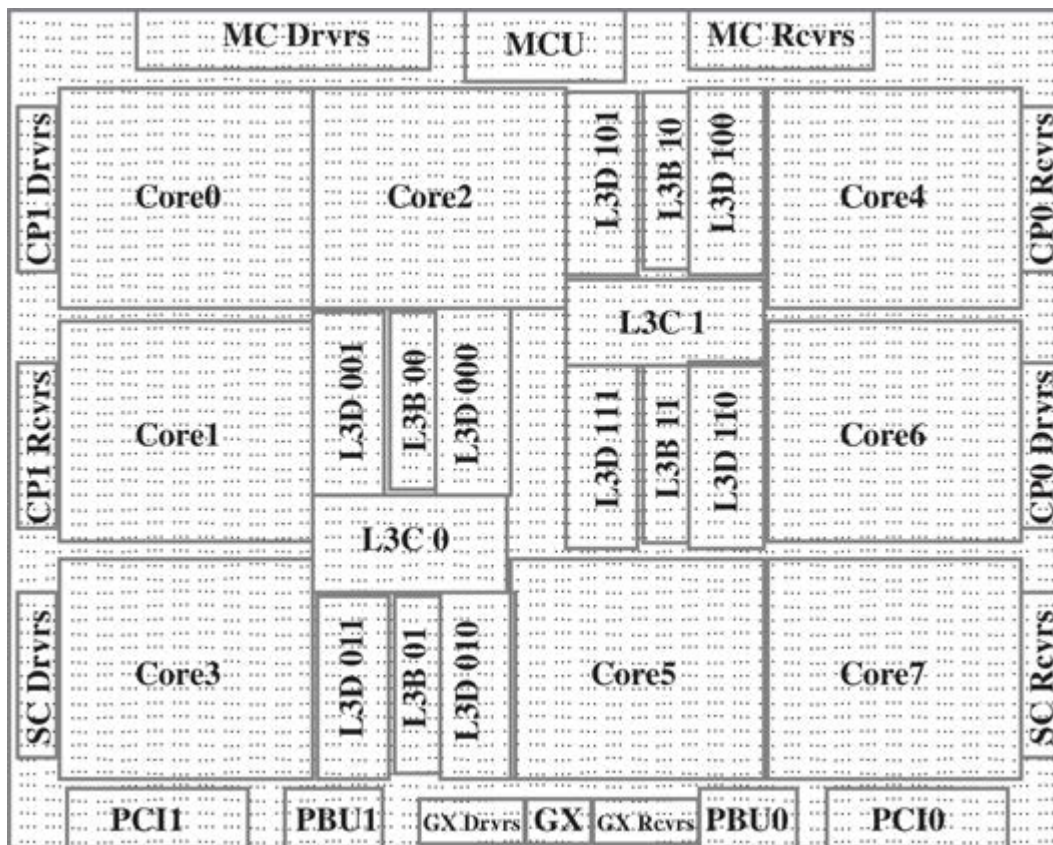
Figure 1.4 IBM z13 Processor Unit (PU) Chip Diagram
