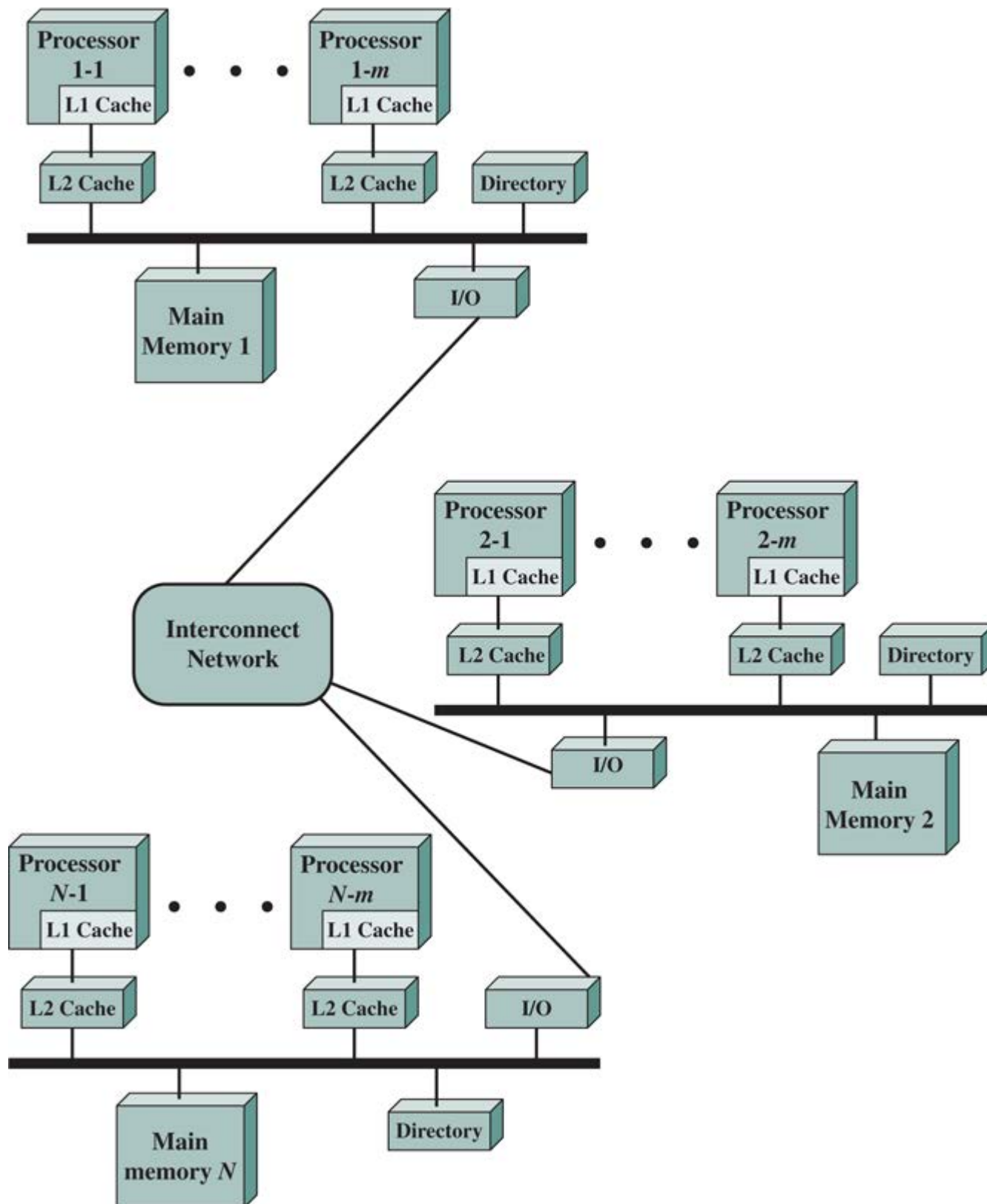
Figure 20.12 CC-NUMA Organization
