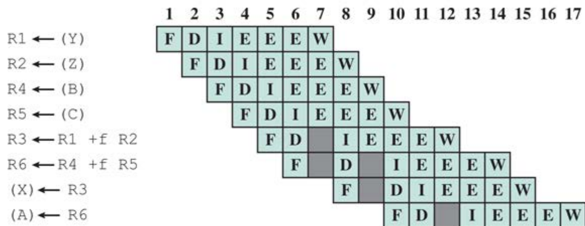
(b) Reorder instruction issuing
