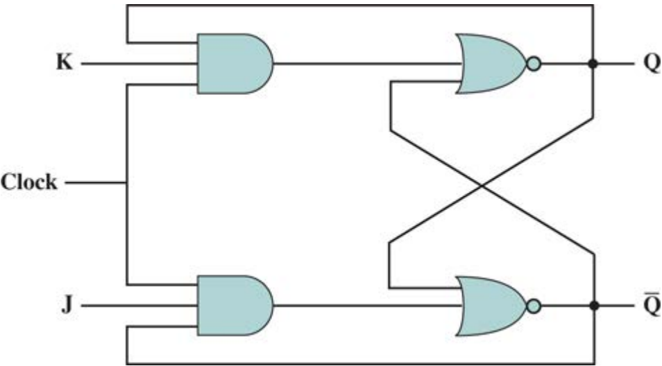
Figure 12.28 J–K Flip-Flop
