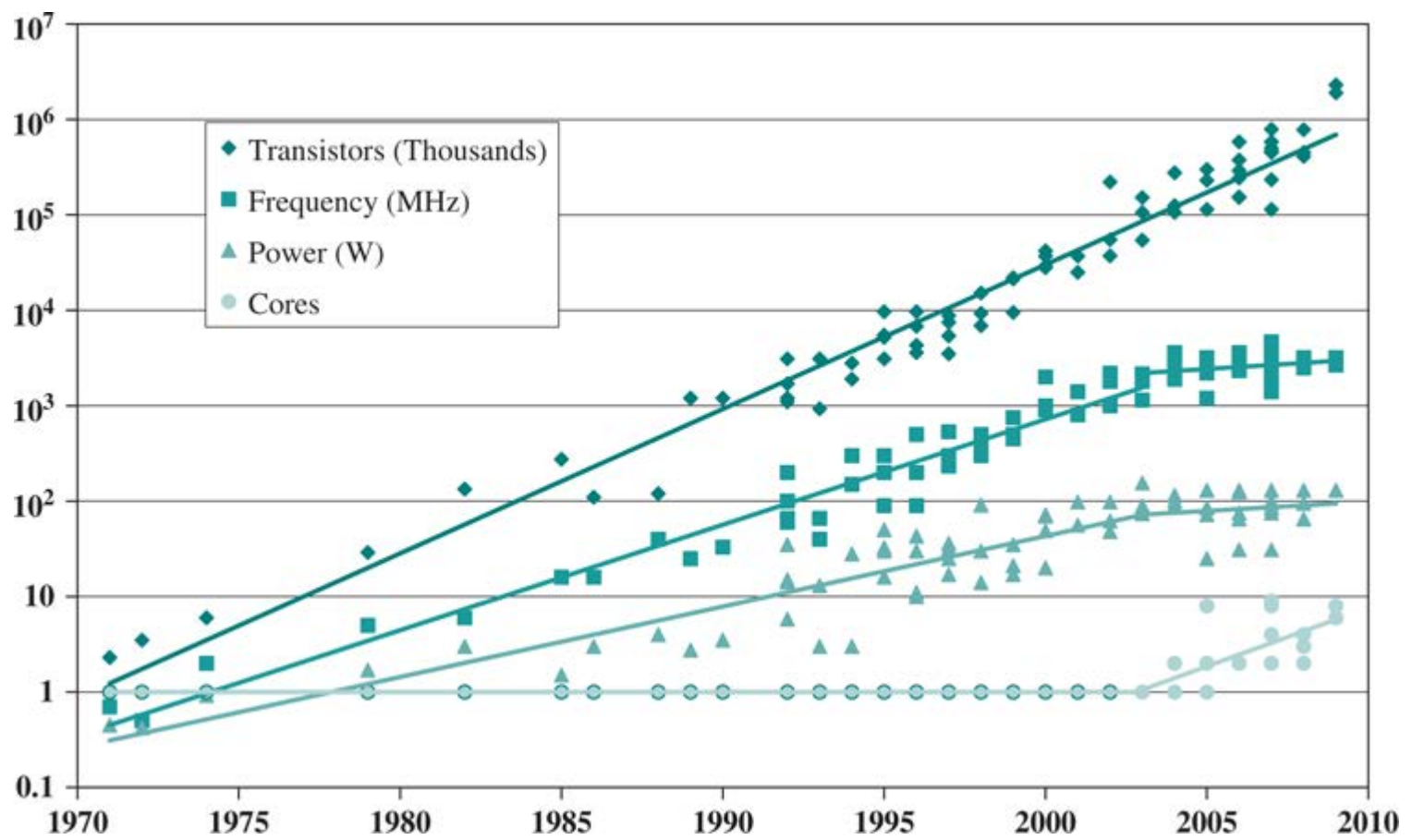
Figure 2.2 Processor Trends
