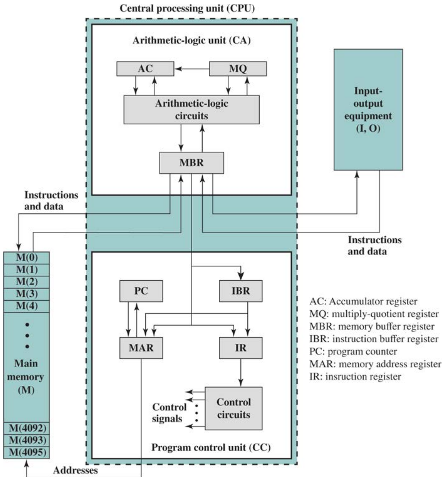
Figure 1.6 IAS Structure
