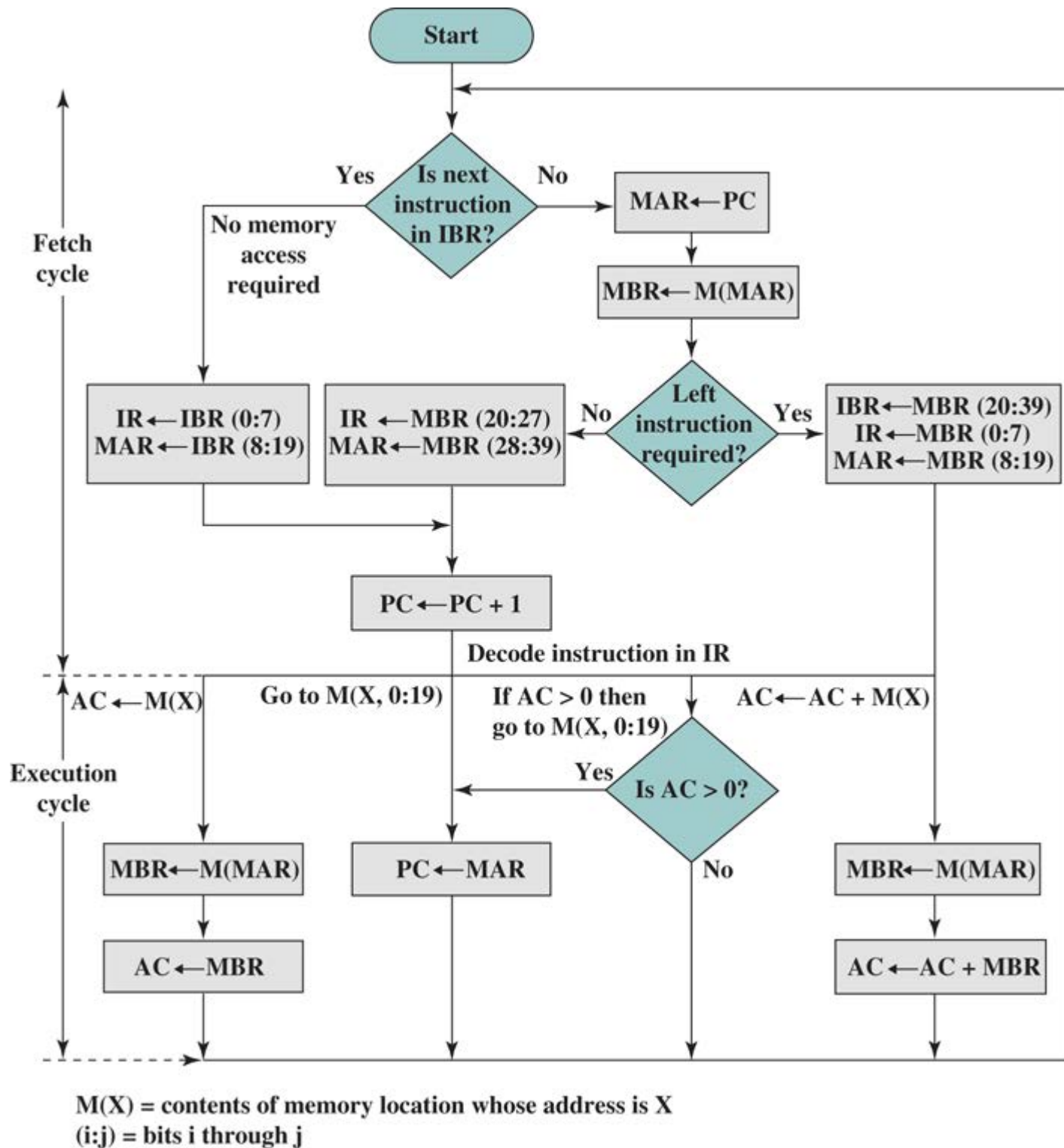
Figure 1.8 Partial Flowchart of IAS Operation
