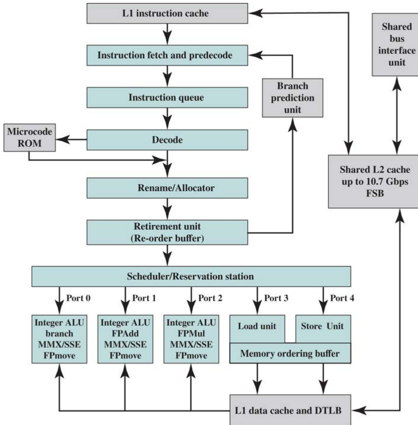
Figure 18.9 Intel Core Microarchitecture
