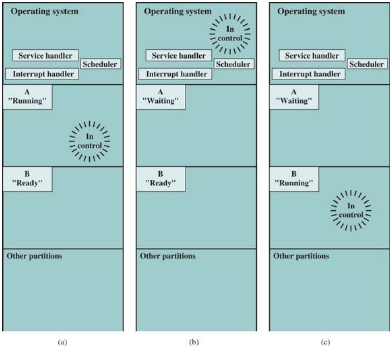
Figure 9.9 Scheduling Example
