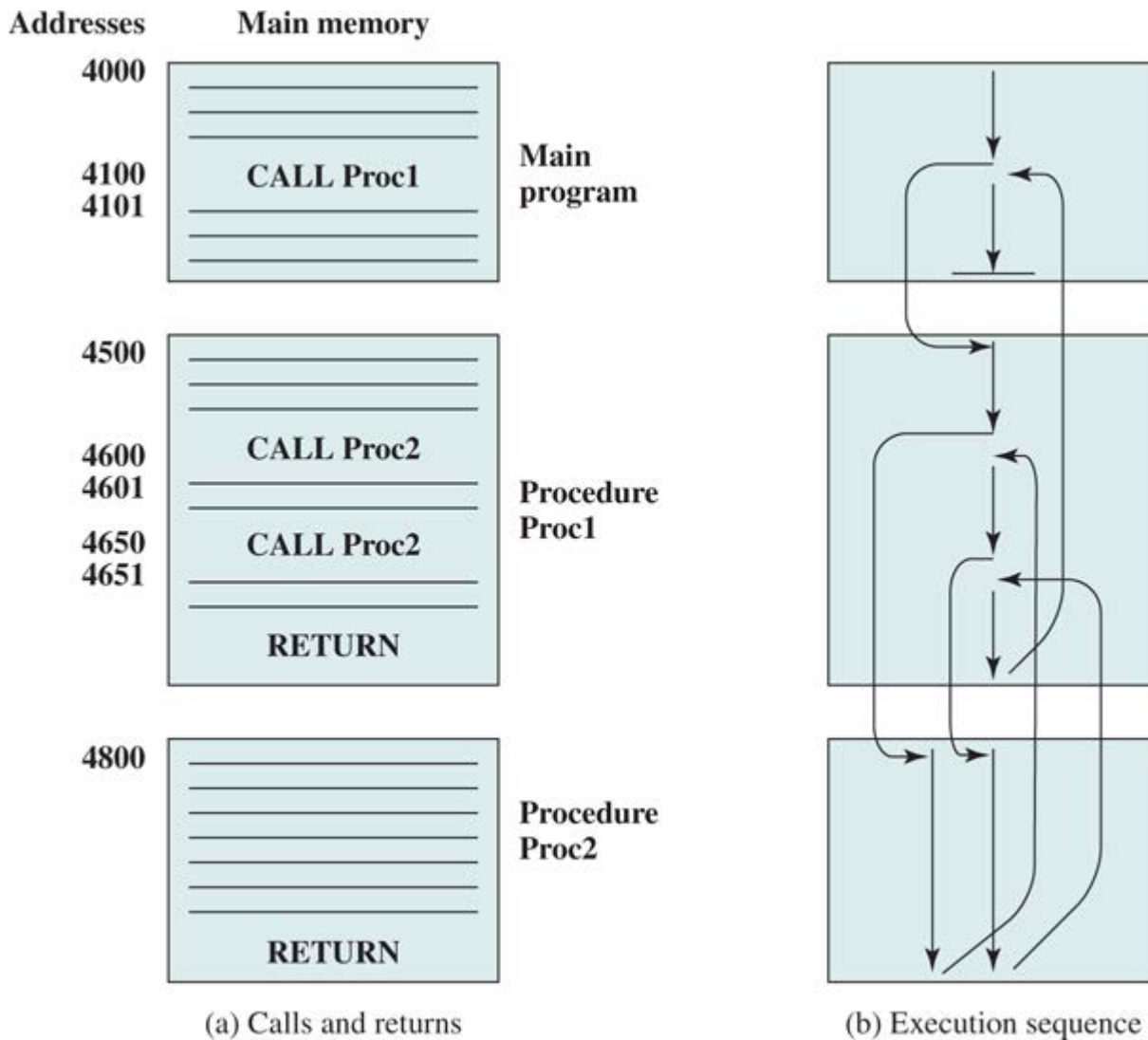
Figure 13.8 Nested Procedures
