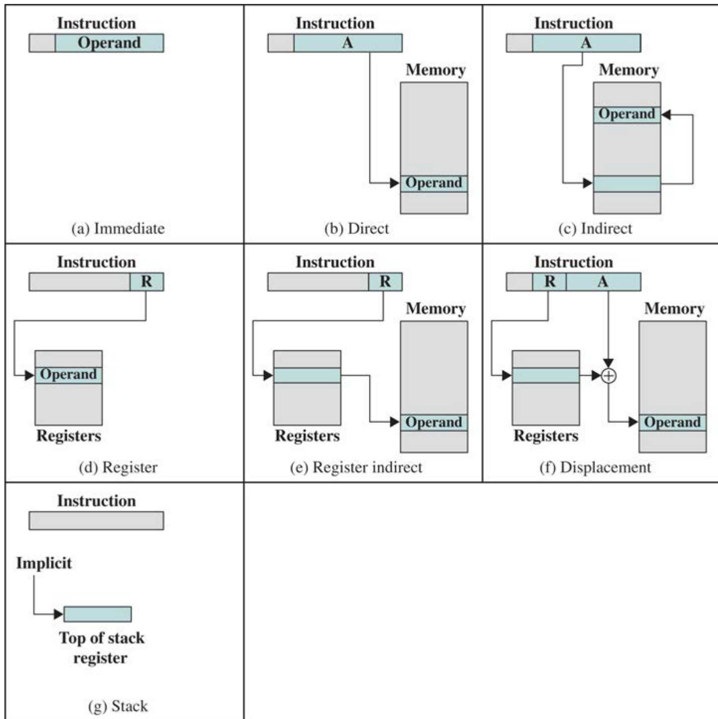
Figure 14.1 Addressing Modes
