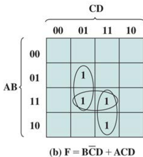
Figure 12.11 Overlapping Groups
