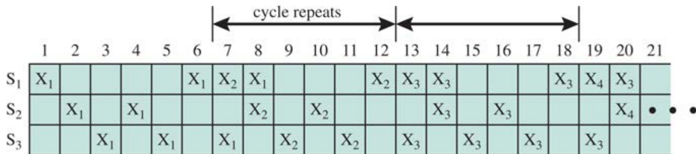
(c) Latency cycle (6) = 6, 6, 6, 6, ... with average latency of 6
