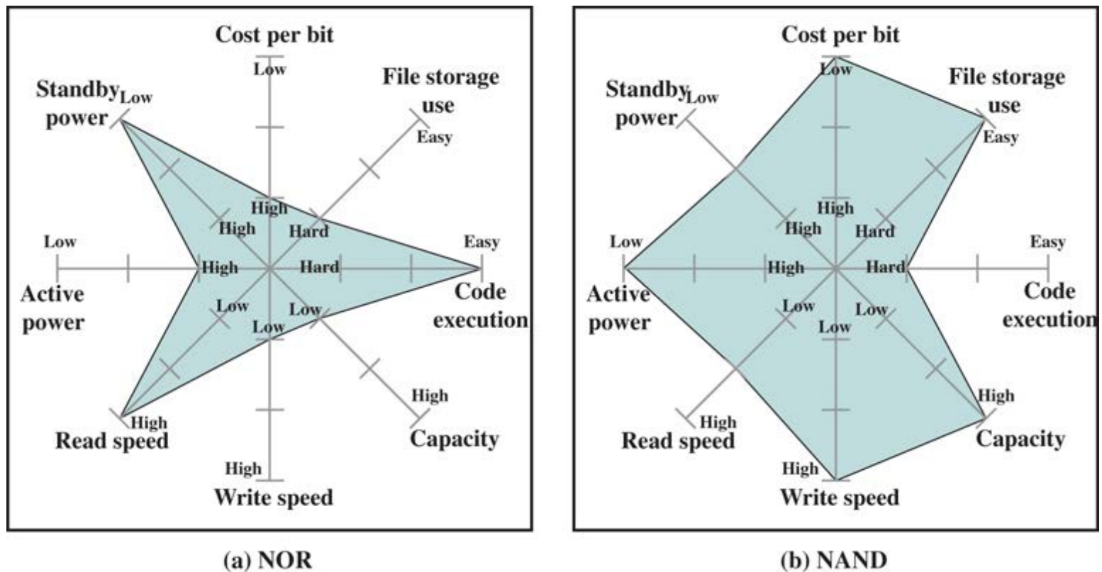
Figure 6.19 Kiviat Graphs for Flash Memory
