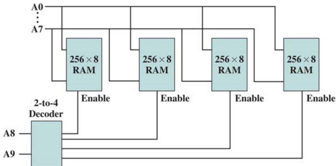
Figure 12.18 Address Decoding
