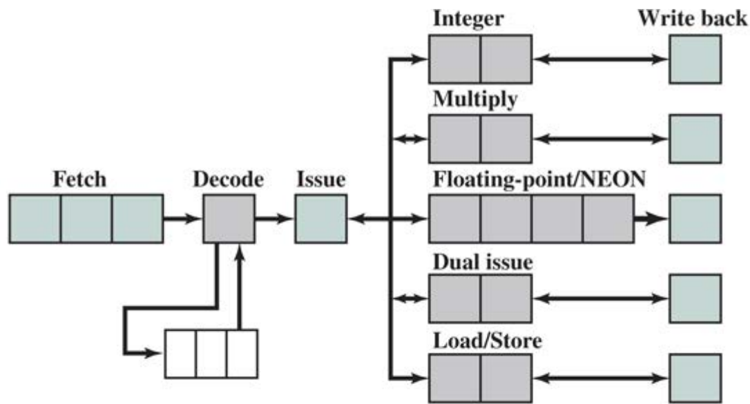
(a) Cortex A-7 Pipeline
