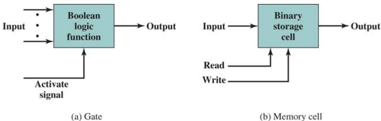
Figure 1.9 Fundamental Computer Elements
