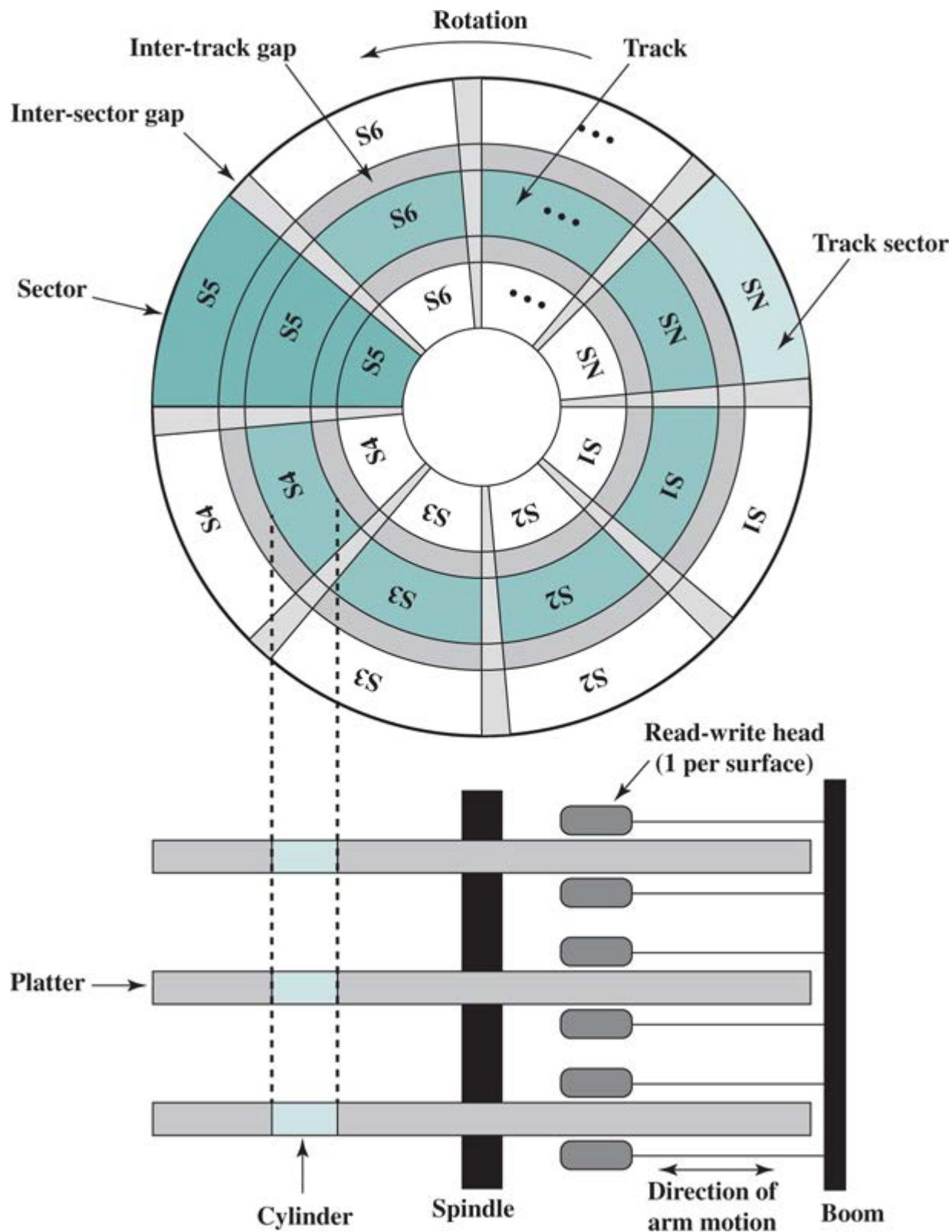
Figure 7.2 Disk Data Layout
