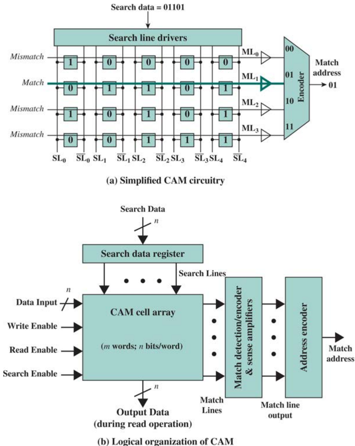
Figure 5.9 Content-Addressable Memory
